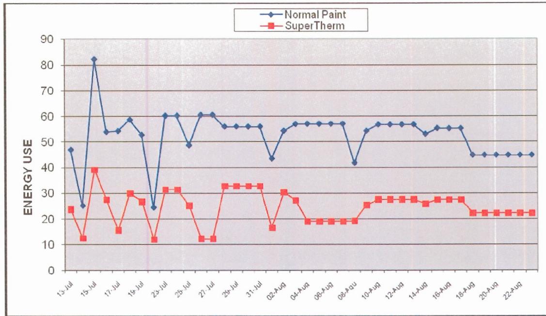
Graph 1: Energy use of containers: one with Super Therm® and one with normal white paint
